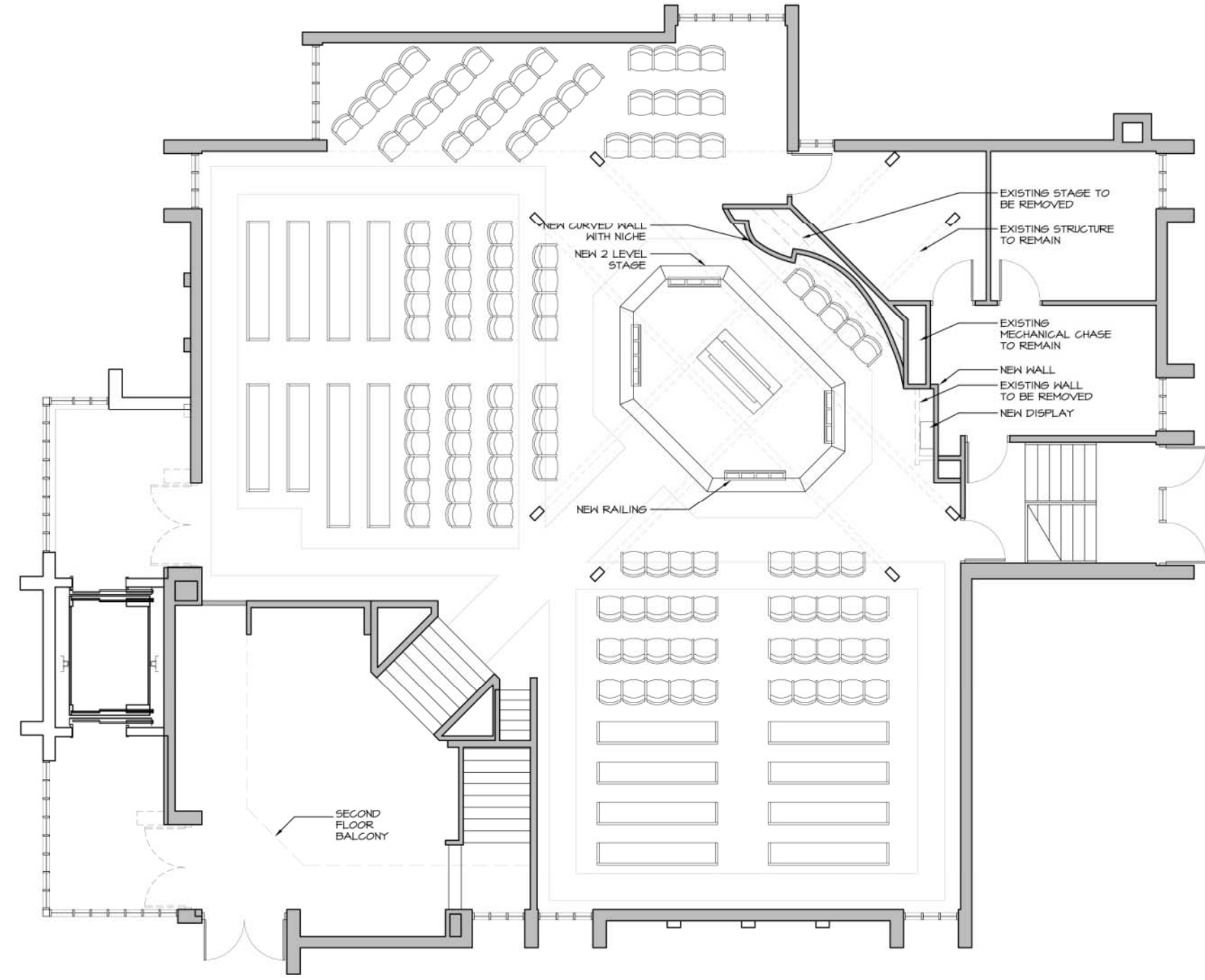
PROPOSED MAIN FLOOR PLAN A2.2.1 SCALE: 1:50
